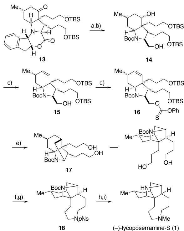
Scheme 5. Completion of the synthesis. a) Red-Al, toluene, 0 °C to RT, 81 %; b) \text{H}_2 , \text{Pd}(\text{OH})_2/\text{C} , \text{Boc}_2\text{O} , \text{EtOAc} , RT, 98 %; c) methoxyacetyl chloride, TMEDA, toluene, RT; \text{ClCH}_2\text{SO}_2\text{Cl} , TMEDA, RT; \text{K}_2\text{CO}_3 , MeOH, reflux, 75 %; d) phenyl chlorothionoformate, DMAP, MeCN, 50 °C; e) V-70, (\text{Me}_3\text{Si})_3\text{SiH} , toluene, 50 °C; CSA, MeOH, RT, 69 % (2 steps); f) \text{MsCl} , TMEDA, \text{CH}_2\text{Cl}_2 , RT, 91 %; g) p\text{NsNH}_2 , \text{Cs}_2\text{CO}_3 , TBAI, DMF, 50 °C, 48 %; h) \text{PhSH} , \text{Cs}_2\text{CO}_3 , MeCN, 50 °C; aq \text{HCHO} , \text{NaBH}(\text{OAc})_3 , RT, 88 %; i) TFA, \text{CH}_2\text{Cl}_2 , RT, 91 %. Boc = tert -butoxycarbonyl, CSA = 10-camphorsulfonic acid, DMAP = 4-(dimethylamino)pyridine, DMF = N,N -dimethylformamide, Ms = methanesulfonyl, Ns = nitrobenzenesulfonyl, Red-Al = sodium bis(2-methoxyethoxy)aluminum hydride, TBAI = tetra- n -butylammonium iodide, TFA = trifluoroacetic acid, TMEDA = N,N,N',N' -tetramethylethylenediamine, V-70 = 2,2'-azobis(4-methoxy-2,4-dimethylvaleronitrile).
